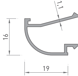
1013 OVAL ISI CAM ÇİTASI 0.190 kg/mt
