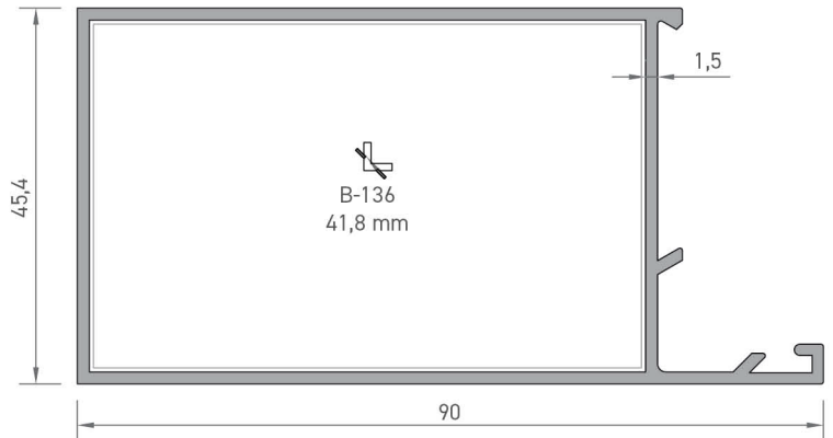
2197 BAZA KASA PROFİLİ 1,025 kg/mt
