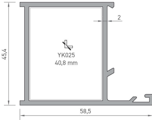
2185 GENİŞ KASA PROFİLİ 1,025 kg/mt
