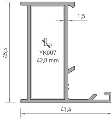
2203 DAR KASA PROFİLİ 0,660 kg/mt
